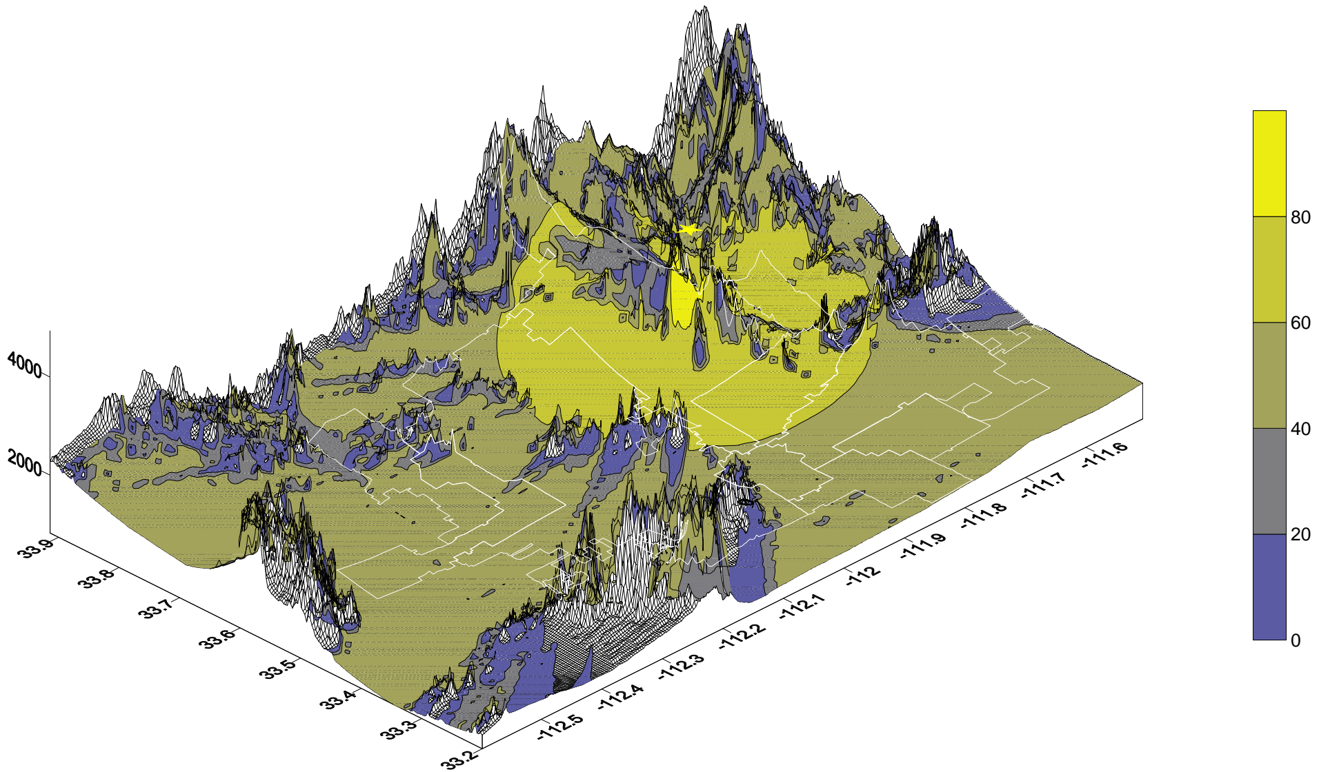
Thompson Peak 800 MHz Predicted Coverage Longley-Rice Poor Conditions (LR 90/90) model ERP=100W Antenna Elevation=50 ft
